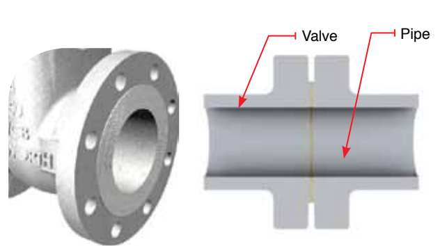
Flanged Ends Raised Face
