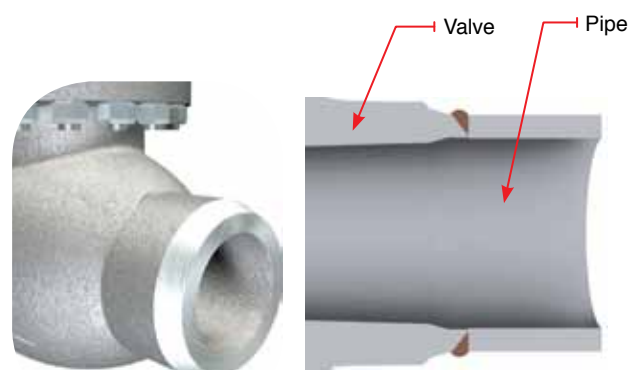
Weld Ends Buttweld
